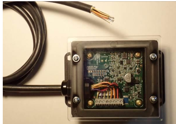
PCB installed unterminated cable in a metal box with 1.5m (AX020720-1.5M)
