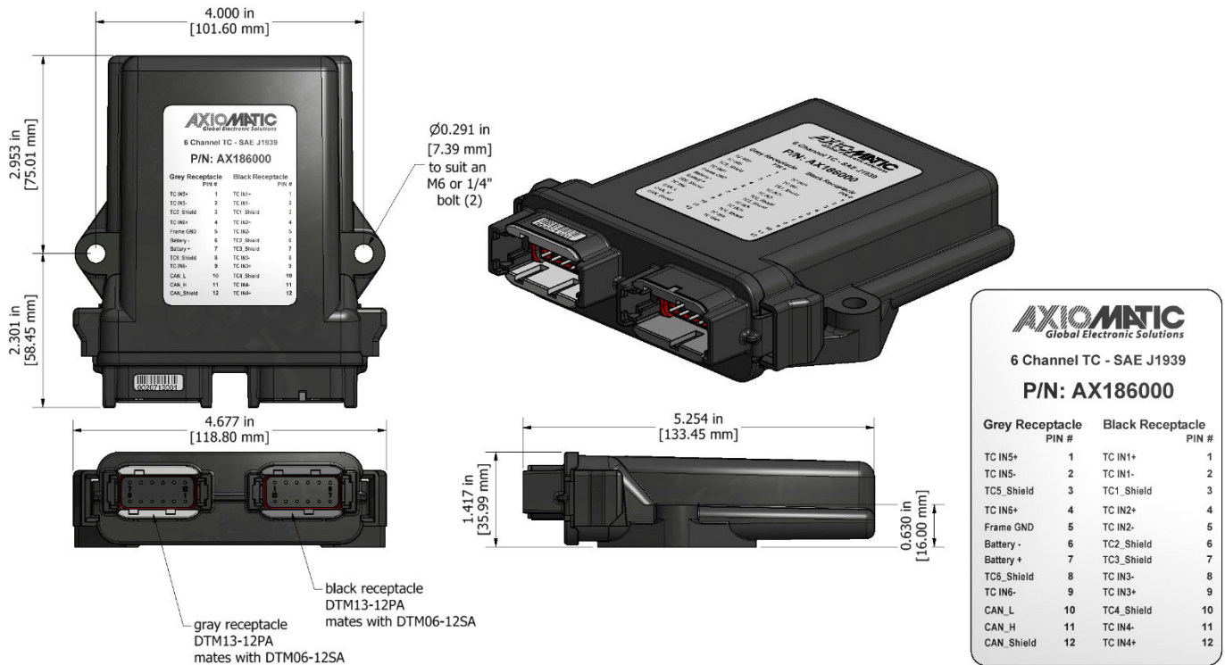
Figure 6 – AX186001 Dimensional Drawing
