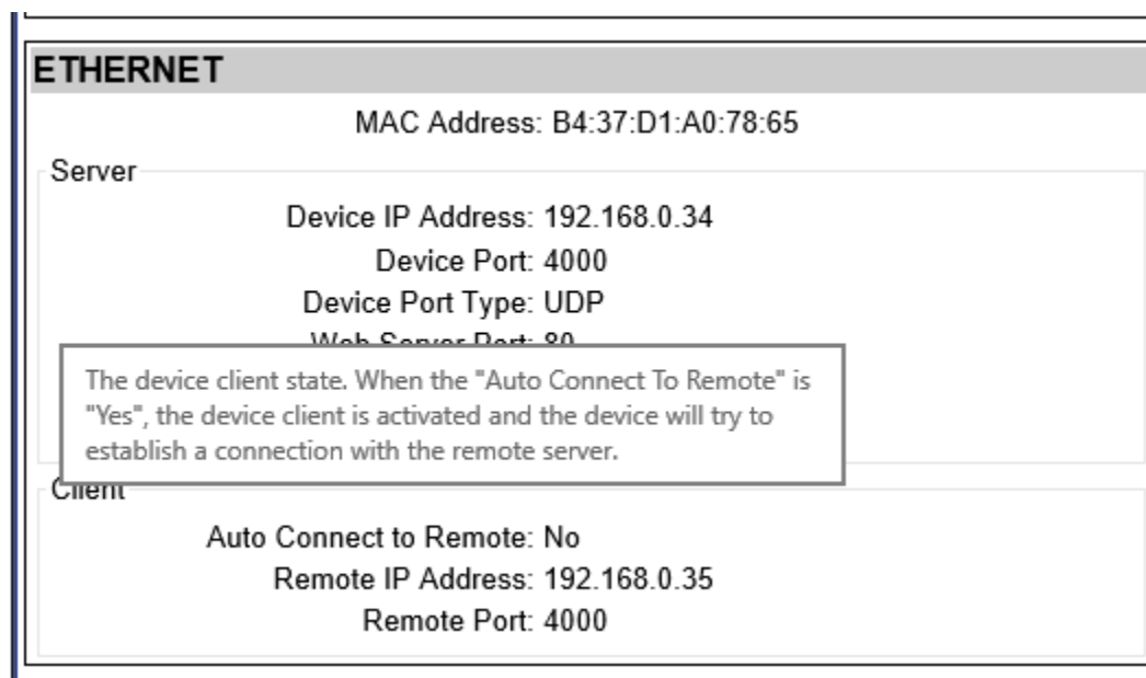
Figure 7. A Tooltip for the "Auto Connect to Remote" Configuration Parameter
