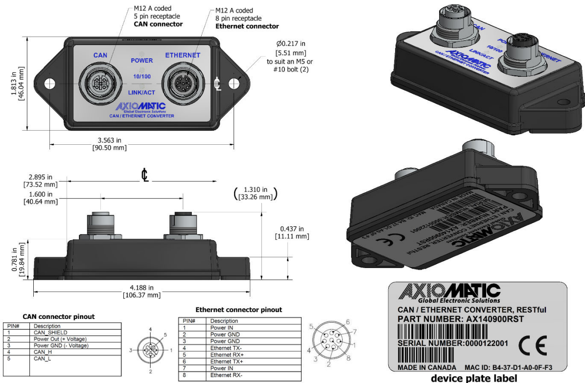
Figure 27. Dimensional Drawing
