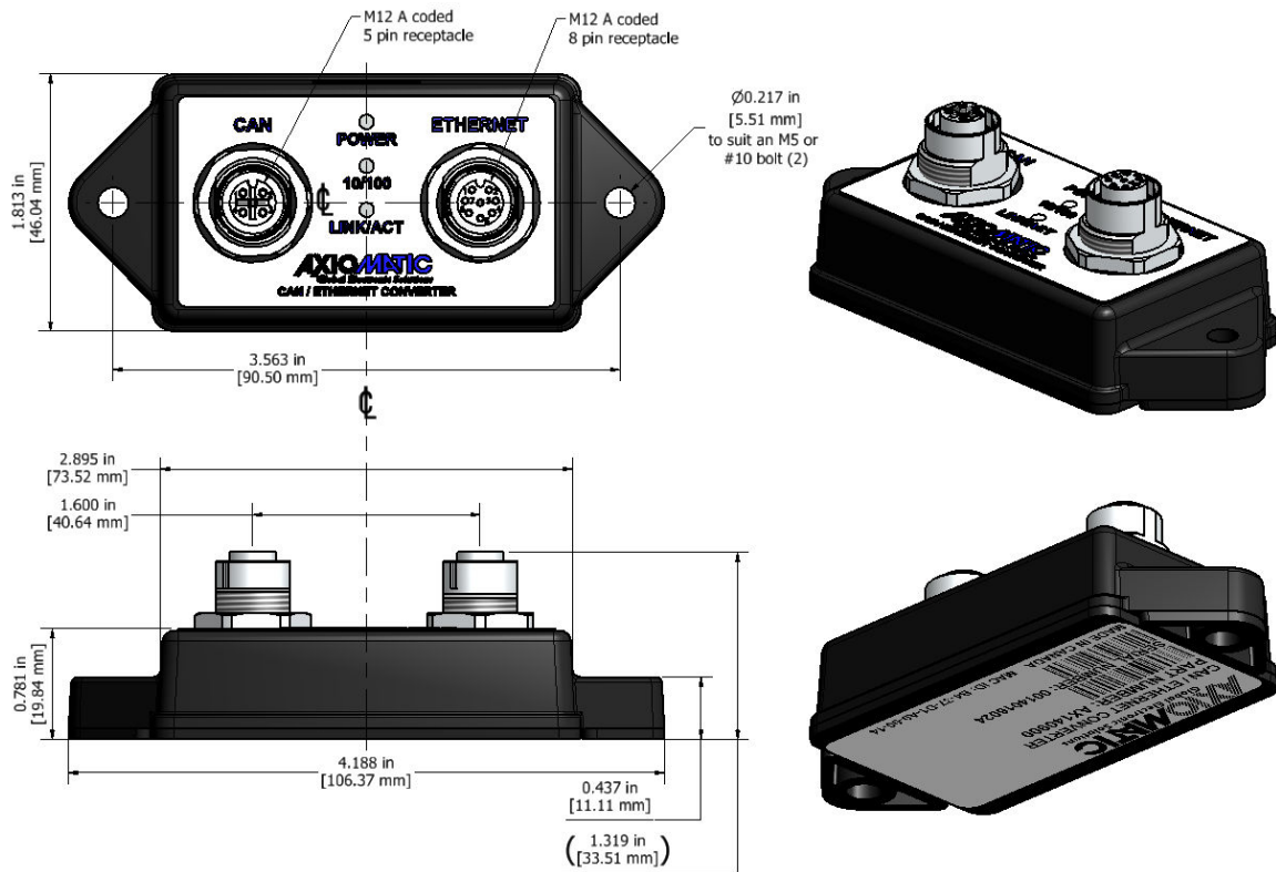
Figure 3.0. Dimensional Drawing
