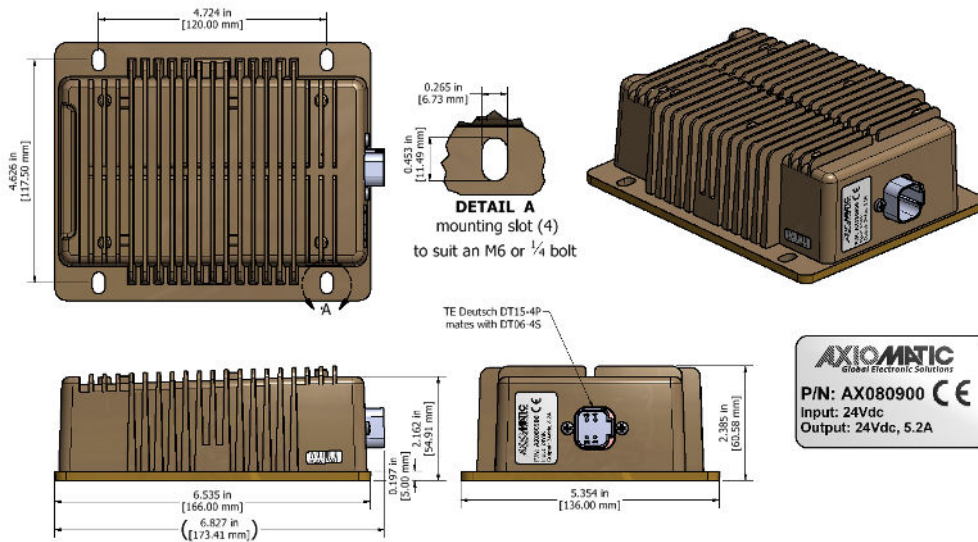
Figure 3.0 – Dimensional Drawing
