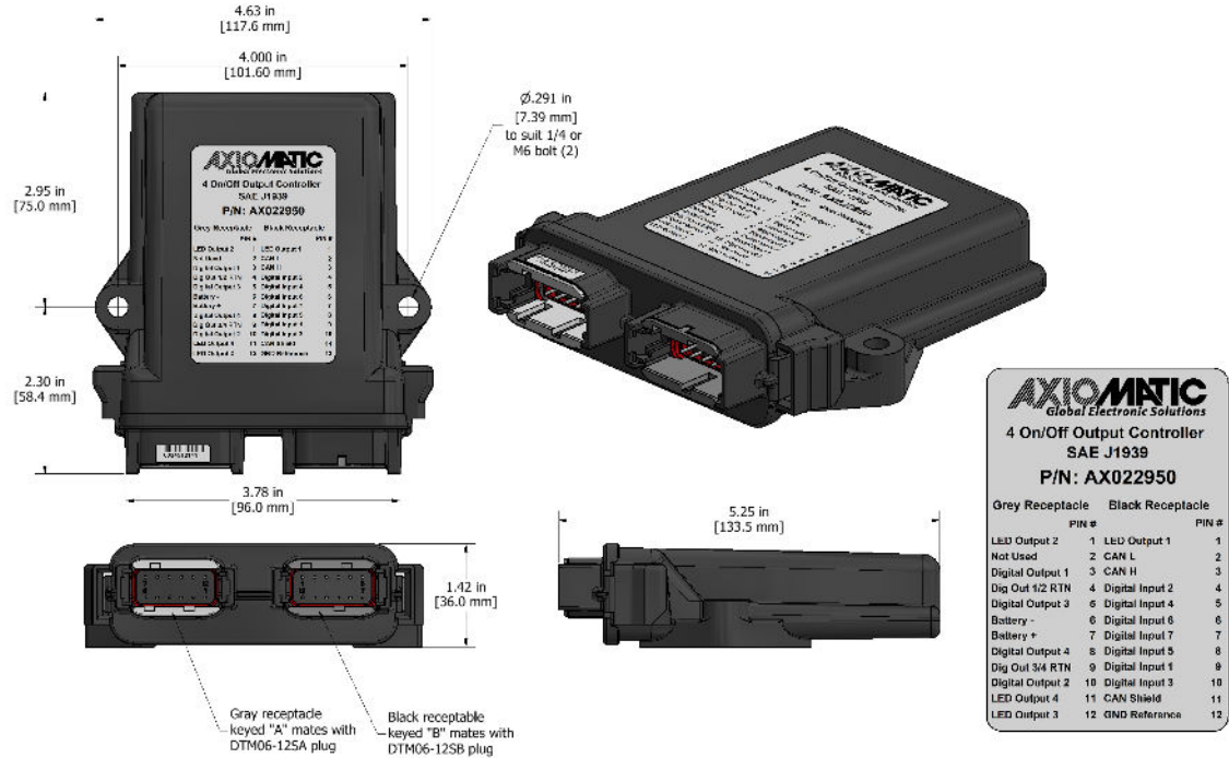
Figure 1.0 – Dimensional Drawing
