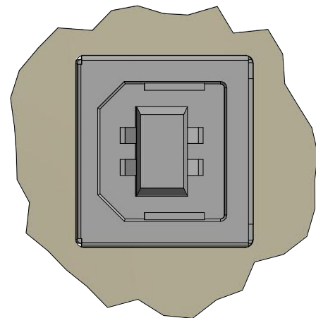
DETAIL A USB receptacle
